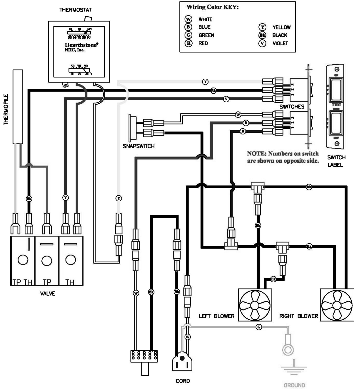
Figure 4: 8890 Wiring Diagram
